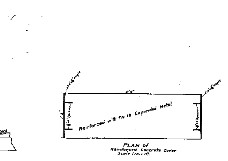
Plan & Sections of Culvert Class No 26
